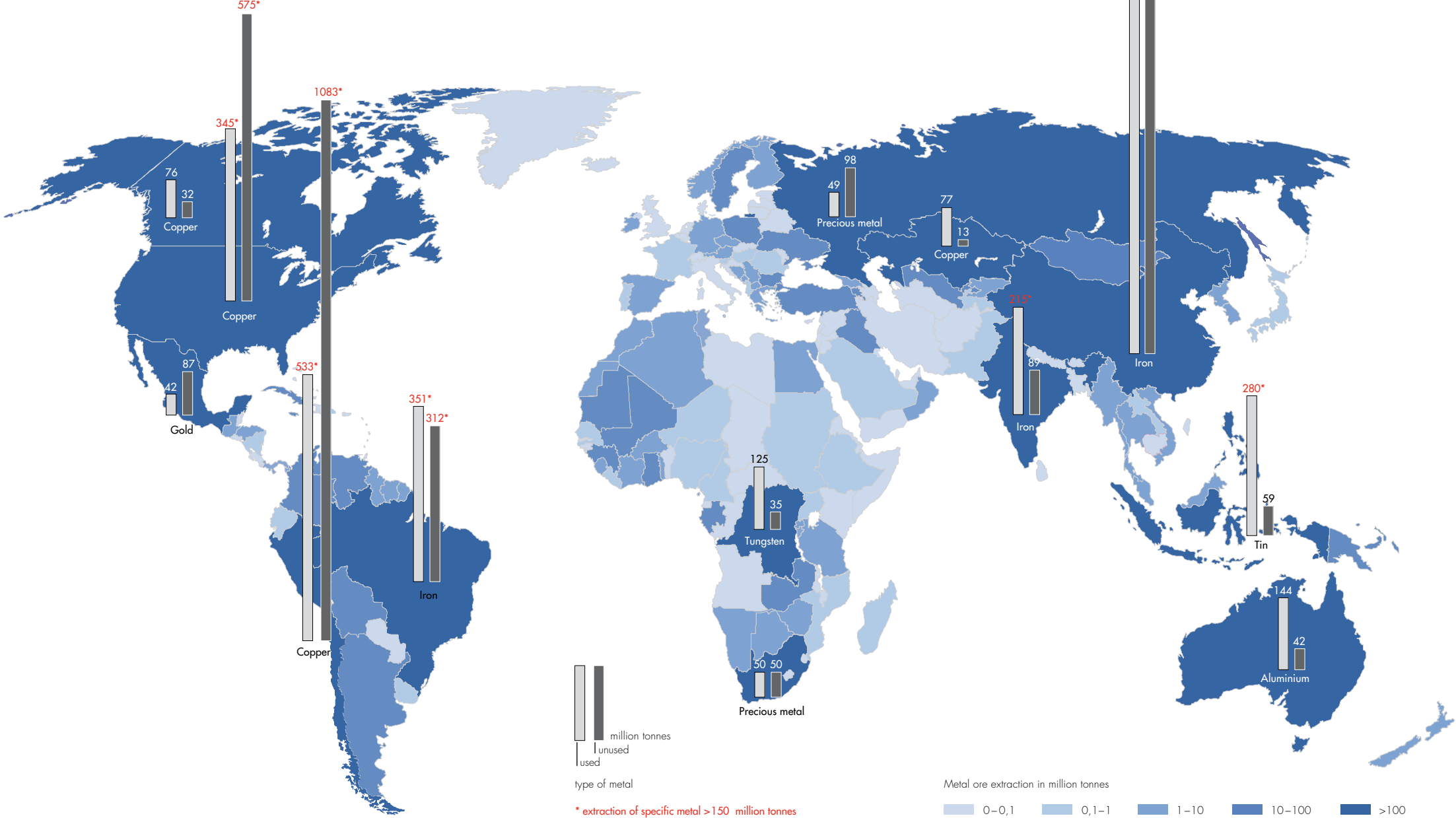
Used extraction of metal ores around the globe combined with examples for used and unused metal extraction 23 in specific countries 2008
