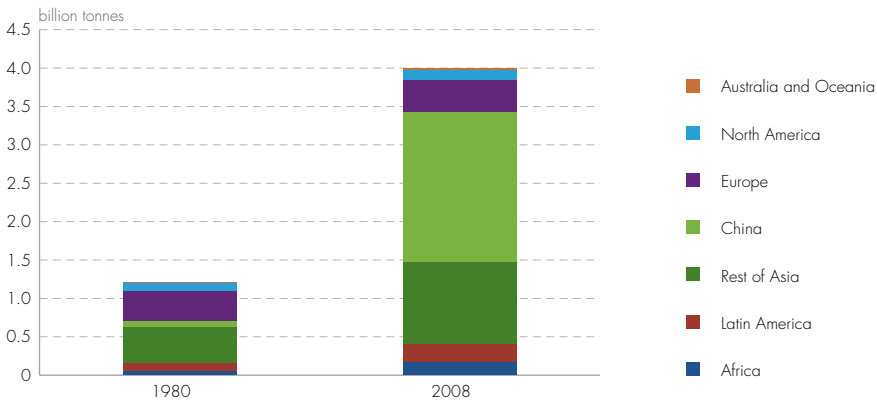
Limestone extraction by continent 1980 and 2008
